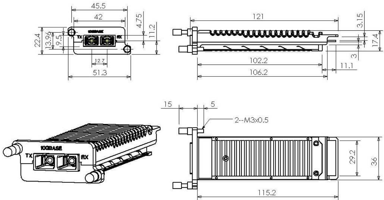
Figure 1 Mechanical dimensions
